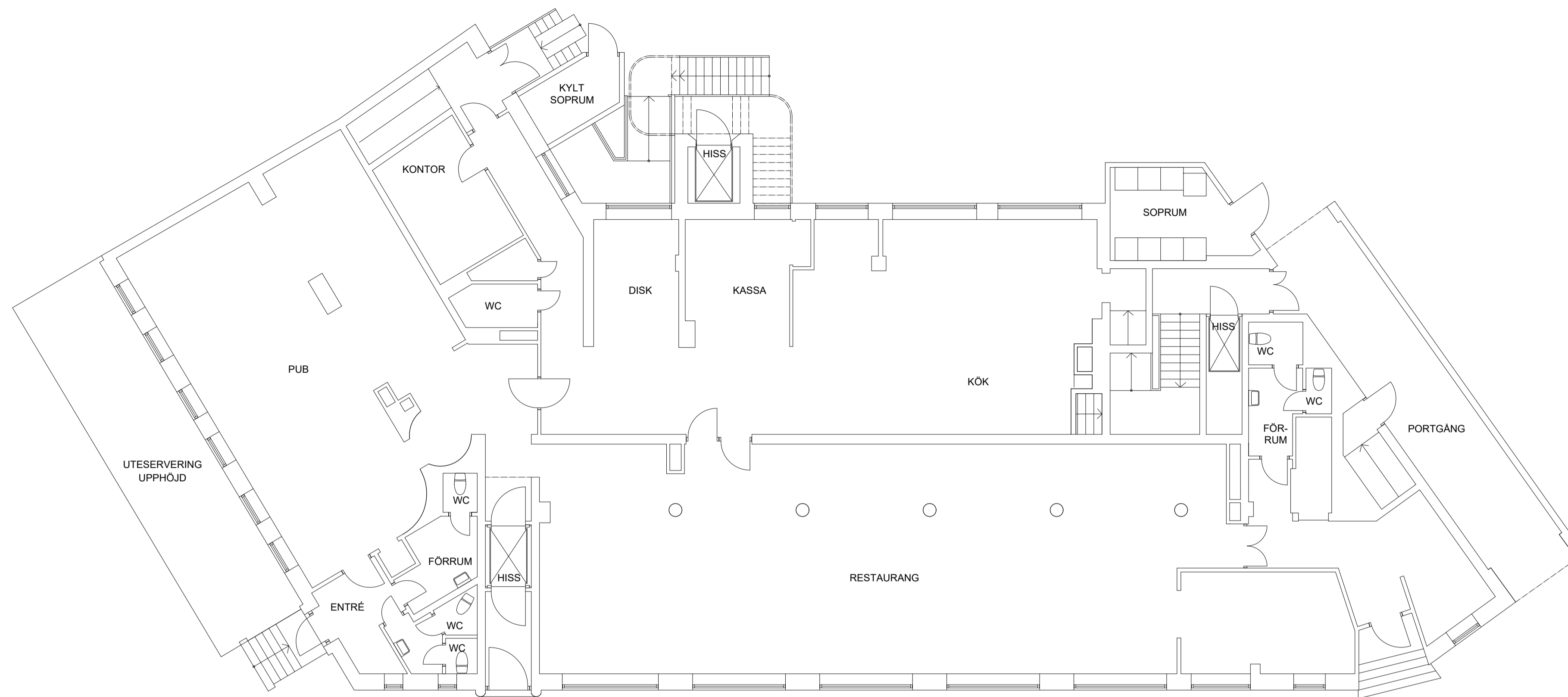
BOTTENPLAN
